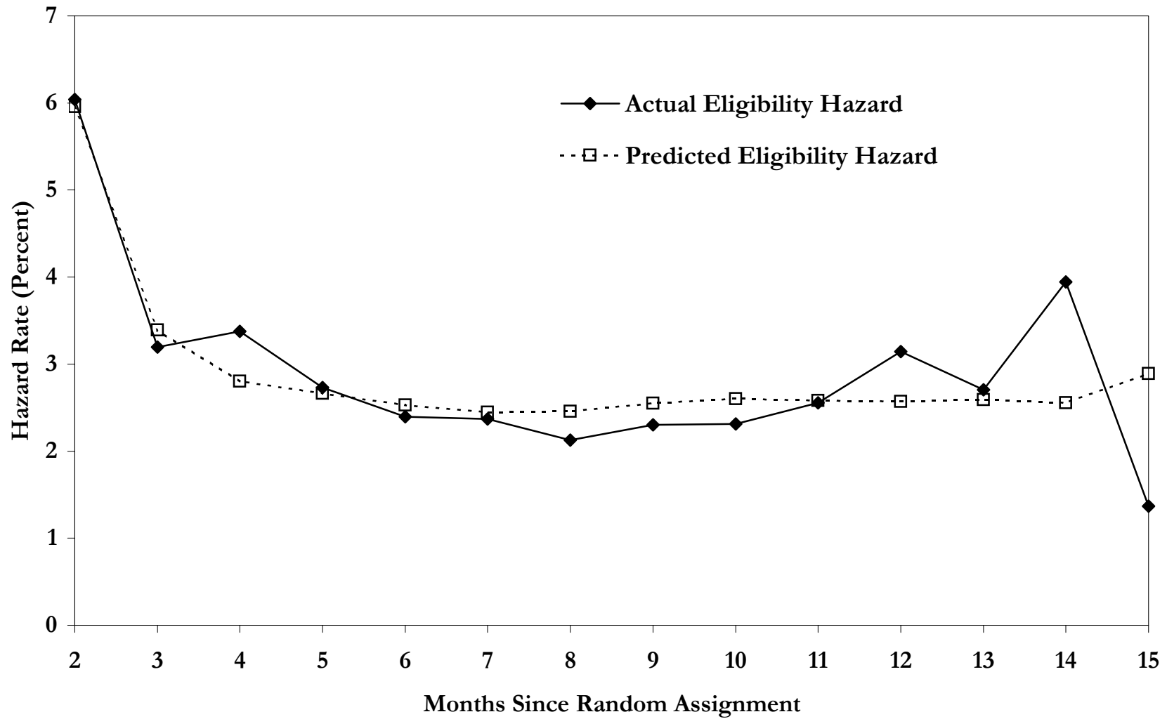
Figure C: Actual and Predicted Hazard into Eligibility
