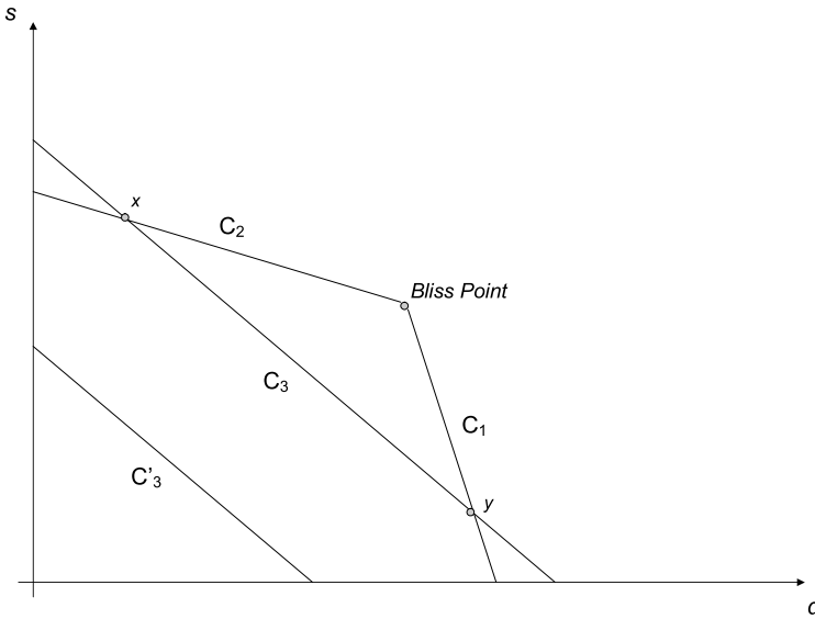
FIGURE S.2.—The loci C_1 , C_2 , and C_3 .
