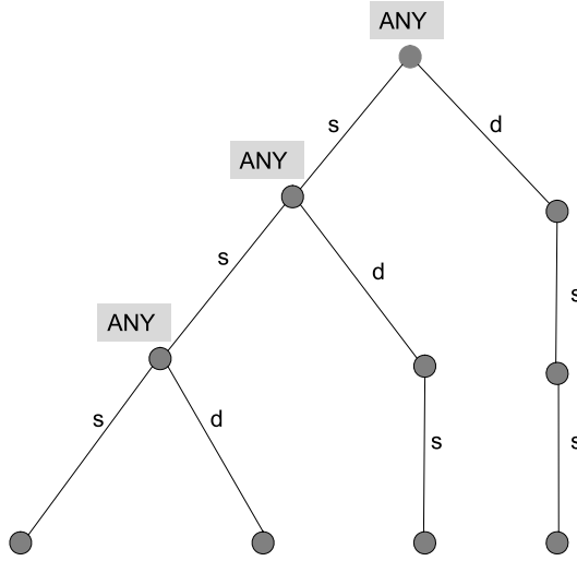
FIGURE S.3.—Tree representation of an equilibrium strategy.
