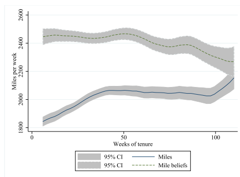
(b) Medians
