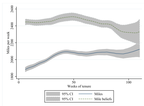
(a) Means
