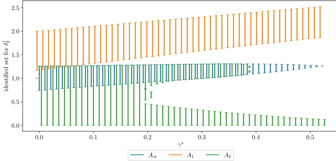
FIGURE 4. \Lambda(F_{\theta, \gamma^*}, A_1) and \Lambda(F_{\theta, \gamma^*}, A_2) at various values of \gamma^* .
