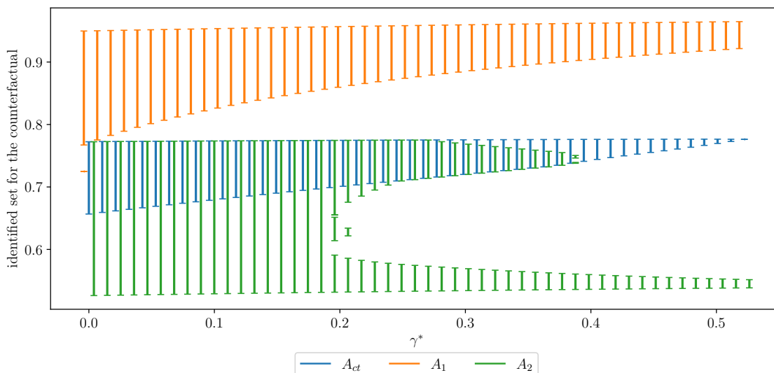
FIGURE 5. \mathbb{P}(Y_1 + Y_2 = 1 | X = x_0) at various \gamma^*
