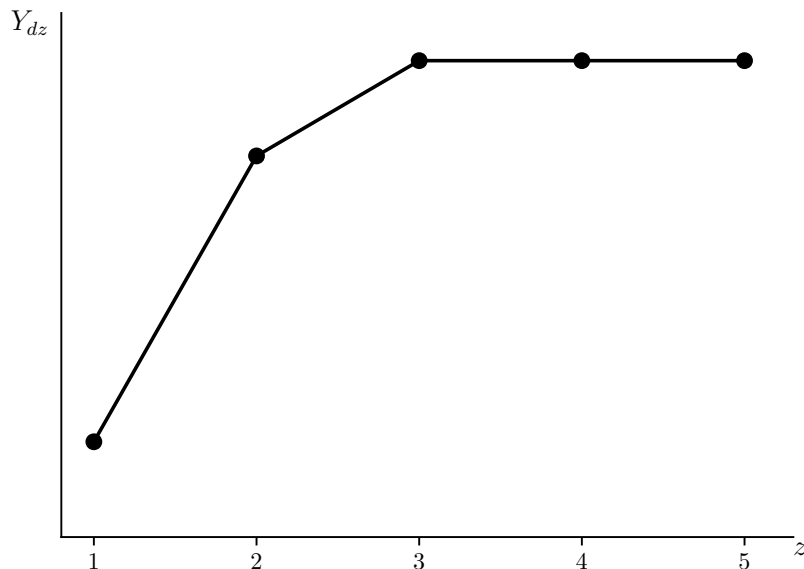
FIGURE 1. Illustration of restriction E.3 when z = 3 and k = 5 .
