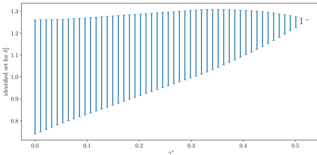
FIGURE 3. \Lambda(F_{\theta, \gamma^*}, A_{ct}) at various values of \gamma^* .
