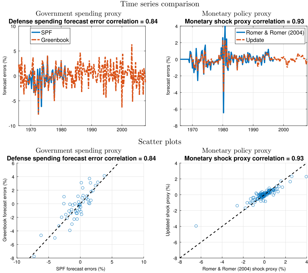
FIGURE B.1. Comparing shock proxies in the literature with their updated counterparts.
