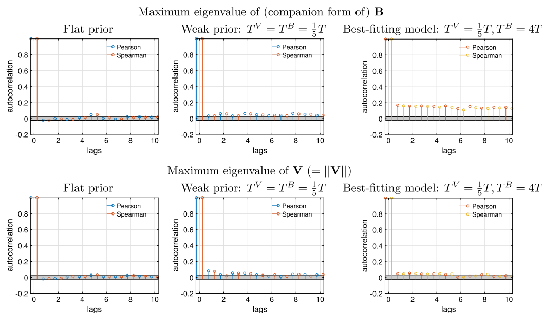
FIGURE B.4. Gibbs sampler of baseline model: Autocorrelation functions of univariate summary statistics by DSGE prior weight. Note: Autocorrelations are reported based on both the Pearson and the Spearman correlation measure. Asymptotic classical 90% credible sets for the Pearson coefficient, computed under the assumption of zero correlation, are included around the horizontal axis. The autocorrelations are based on the thinned out sample after keeping every 20th draw with the informative prior and every 10th draw with the flat prior. The resulting sample is reasonably efficient also with a larger prior weight on the DSGE model.
