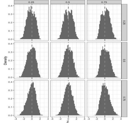
(b) \epsilon_{i,t} \sim Cauchy , T = 50,000
