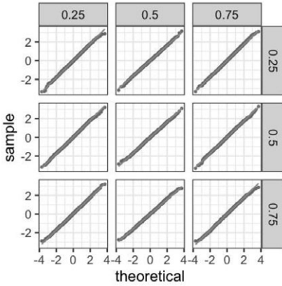
(a) \epsilon_{i,t} \sim N(0, 1) , N = 100 , T = 10
