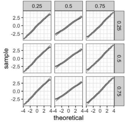
(b) \epsilon_{i,t} \sim Cauchy , N = 50,000
