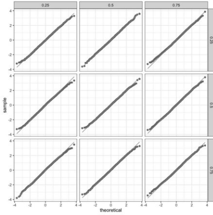
(a) \epsilon_{i,t} \sim N(0, 1) , N = 100
