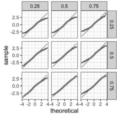
(b) \epsilon_{i,t} \sim Cauchy , T = 50,000
