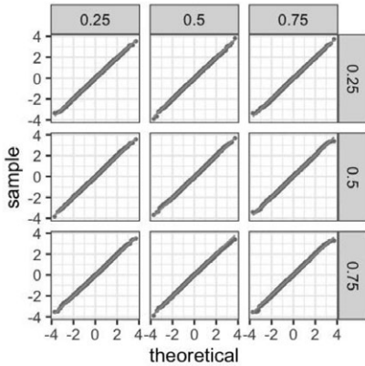
(a) \epsilon_{i,t} \sim N(0,1) , T = 100
