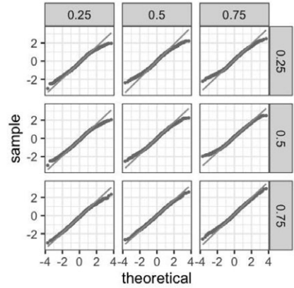
(b) \epsilon_{i,t} \sim Cauchy , N = 500 , T = 100
