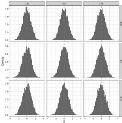
(a) \epsilon_{i,t} \sim N(0, 1) , N = 100
